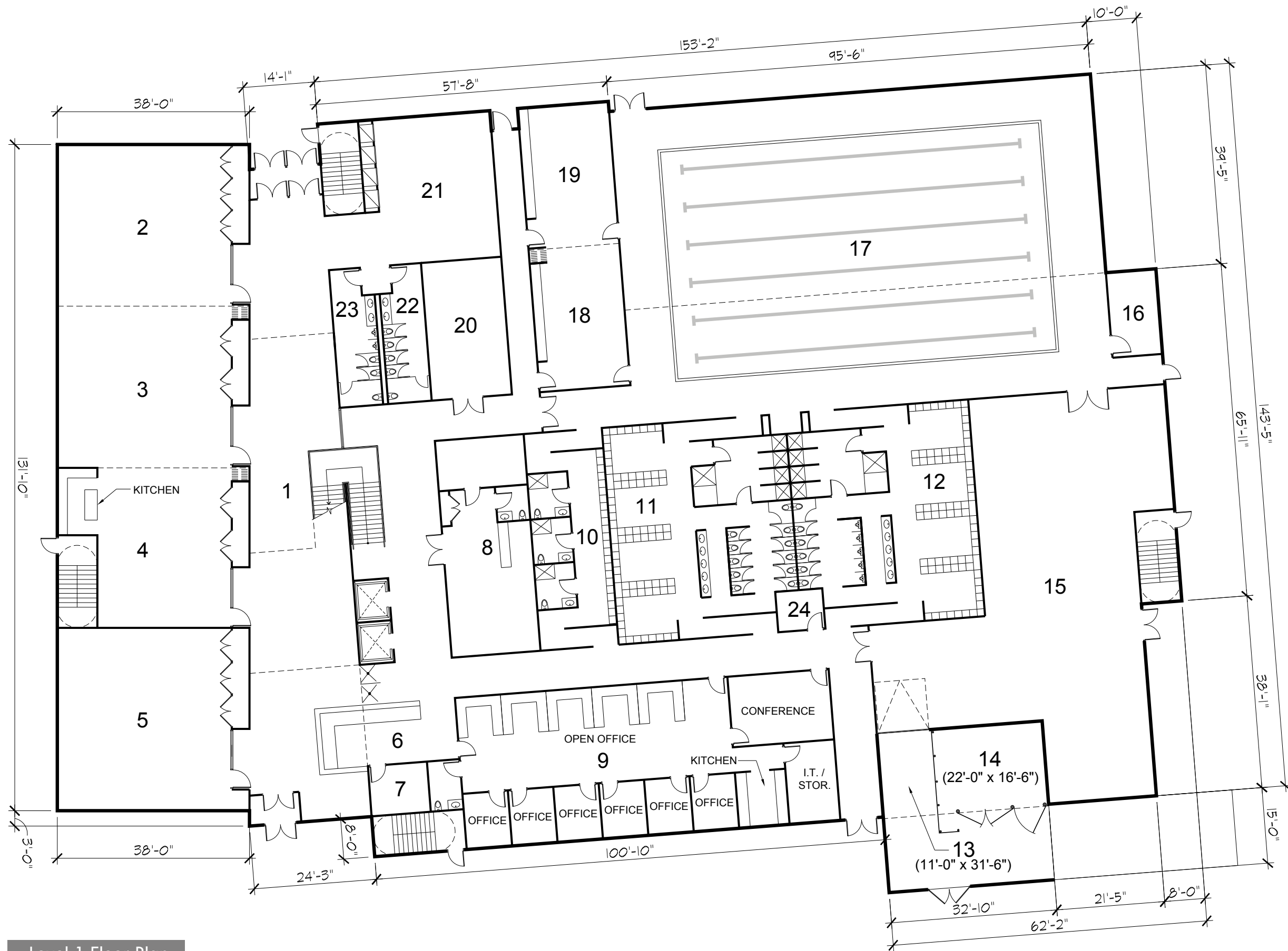
Level 1 Floor Plan
